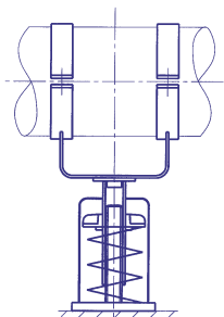
Spring support, type 29
