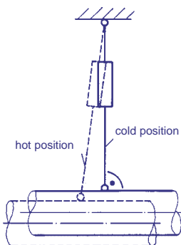
Case 2 Attachment rods vertical in installation condition
