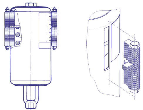
Blocking device for single spring models
